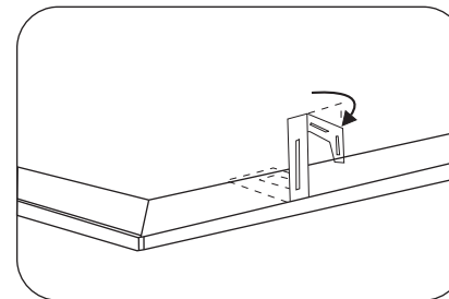
③ Turn the mounting clip head
