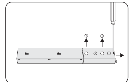
⑥ Remove the driver box cover.
