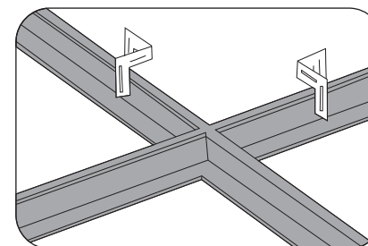
⑤ Check the clips well fasten to T-BARM (Main/Cross ceiling tee.)
